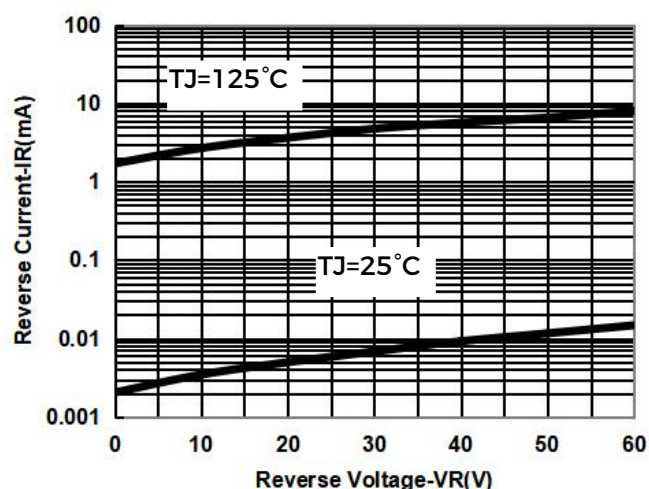
Fig.2-Typical Reverse Characteristics
