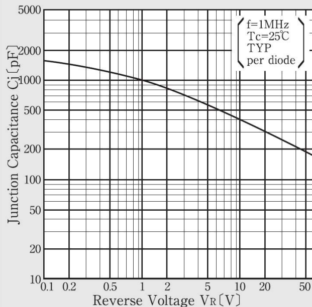
Junction Capacitance
