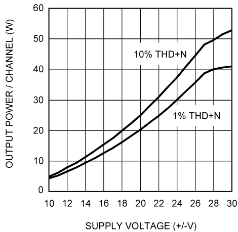
Output Power/Channel vs Supply Voltage f = 1kHz, R L = 6Ω, 80kHz BW
